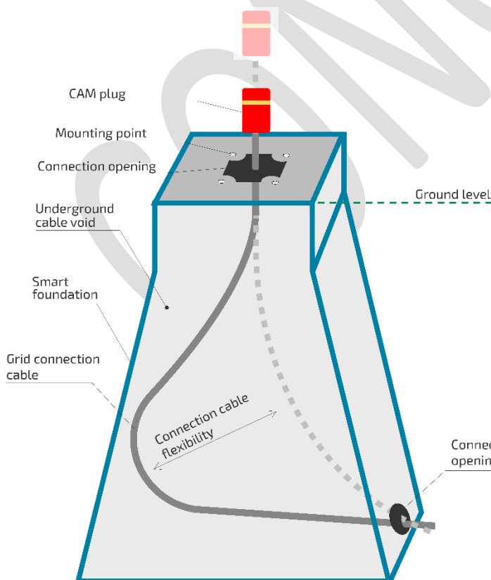
Figure 2 Cross-section of an example of a smart foundation in which properties such as the flexibility of the connection cable are visualised.
