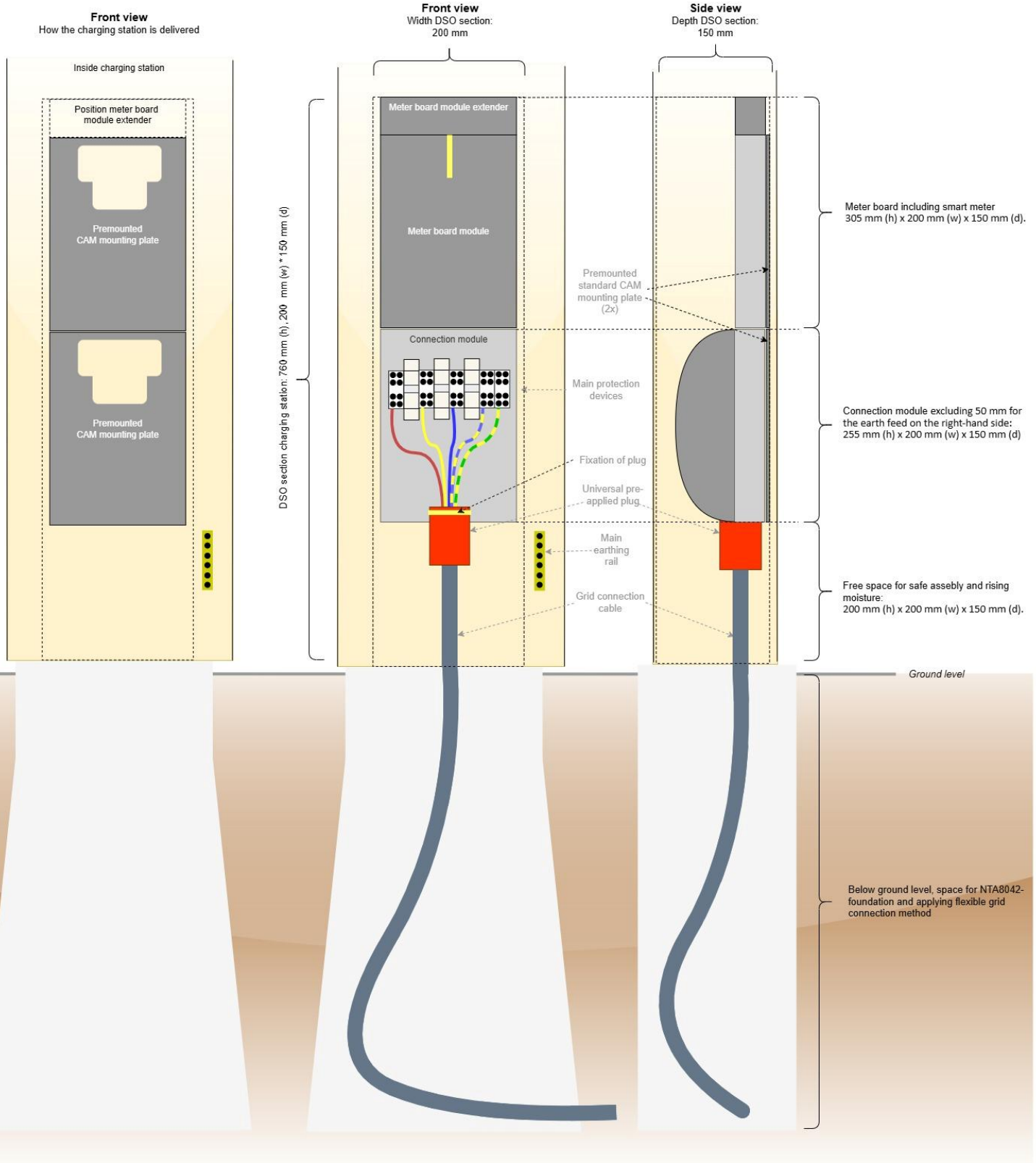
Figure 1: layout and dimensions of the DSO section and the introduction of a grid connection cable with a smart foundation.
