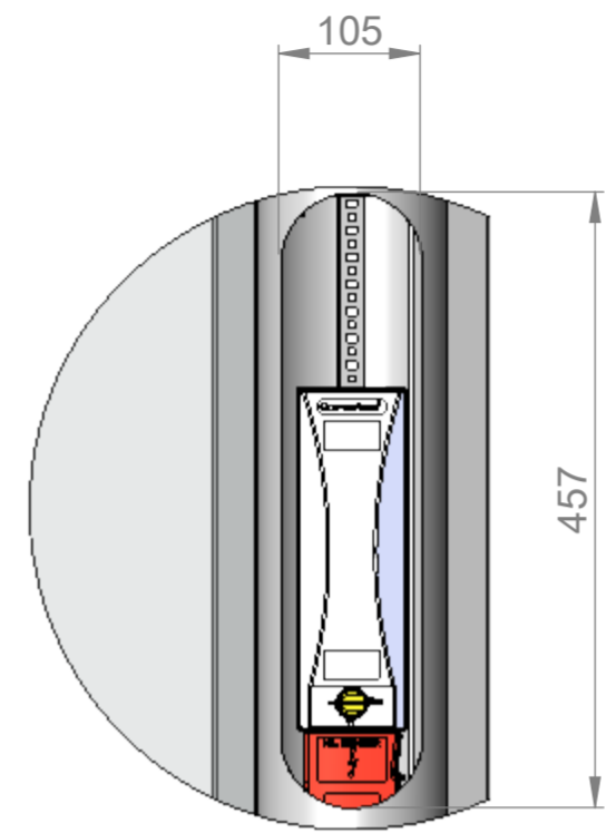
DETAIL D SCALE 4 : 25
