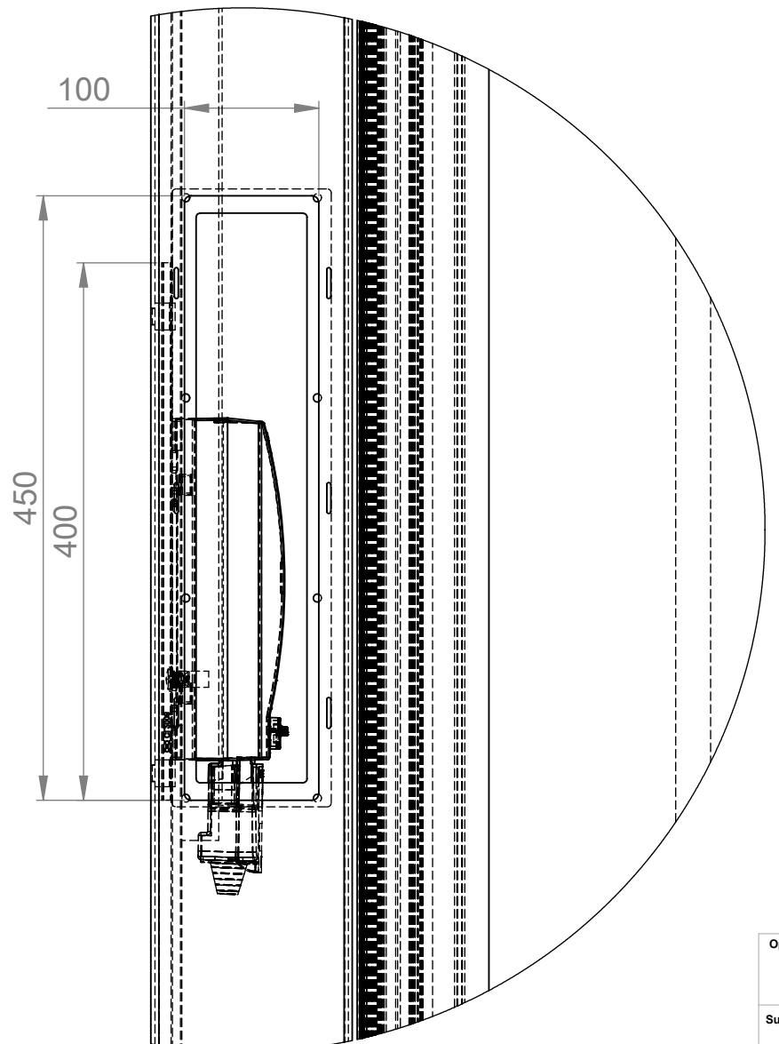
DETAIL B SCALE 1 : 5
